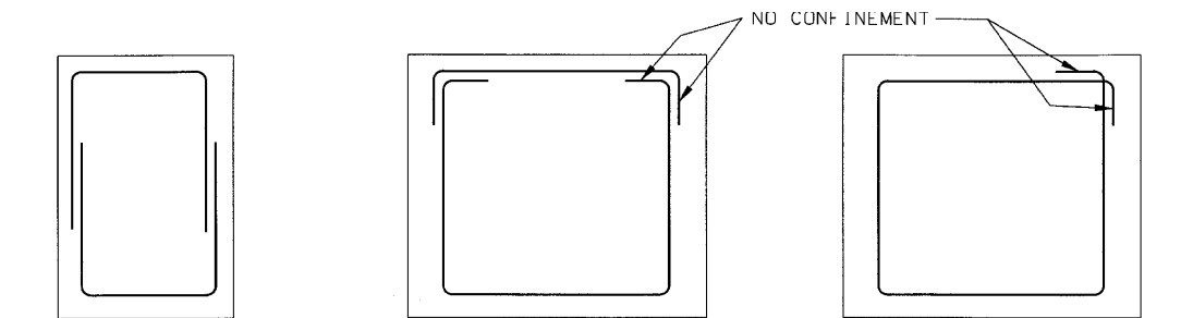
INEFFECTIVE CLOSED STIRRUP STYLES WHICH SHOWED PREMATURE FAILURE IN TESTS UNDER PURE TORSION
