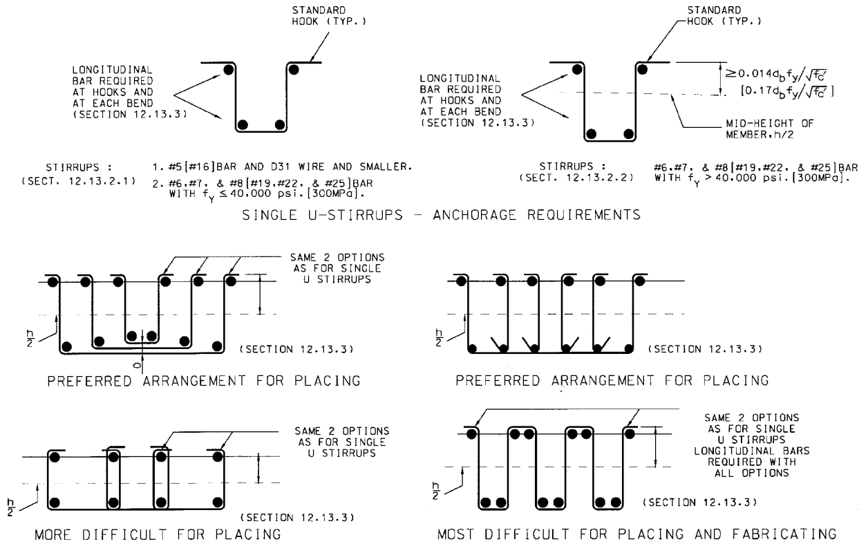
Fig. 11—ACI requirements for anchorage of open stirrups.
